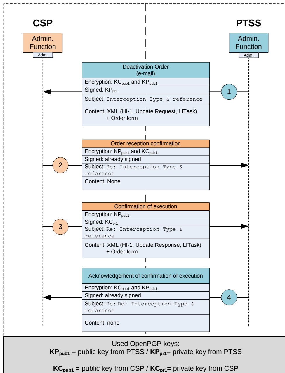
Figure 4-13: Message flow for email deactivation order processing for real-time interceptions
