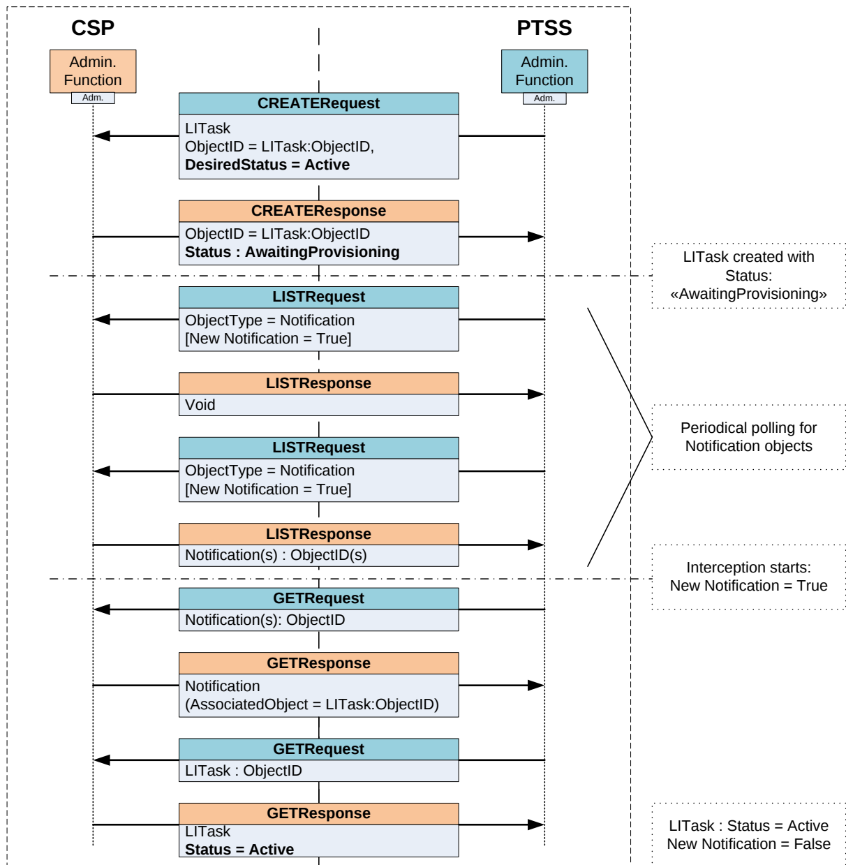
Figure 4-2: Message flow for a real-time interception activation order based on HTTP
